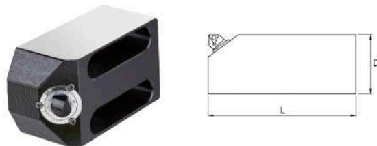
BLB 刀盤 BORING BLOCK/BLB
