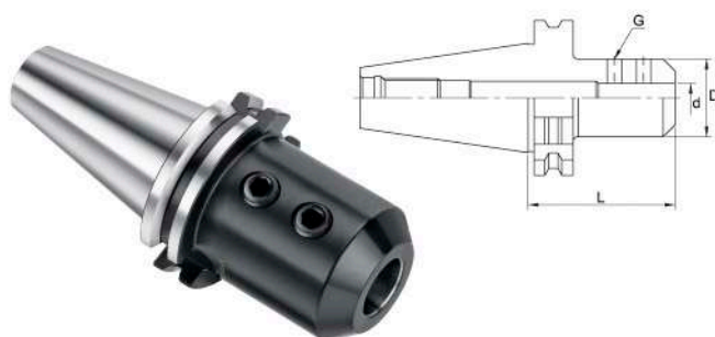
SLA 側固式立銑刀柄 SIDE LOCK END MILL HOLDER/SLA
