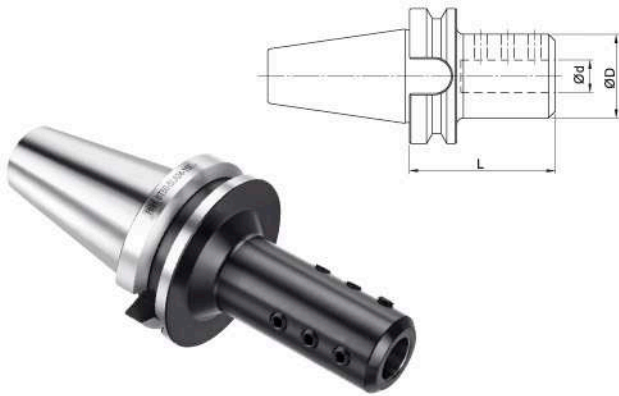
SLA 鎢鋼柄專用側固式刀桿 SIDE LOCK HOLDER FOR CARBIDE TOOL/SLA
