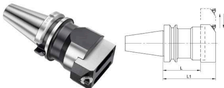
BLB 大口徑微調刀柄 LARGE SIZE MICRO BORING HOLDER/BLB
