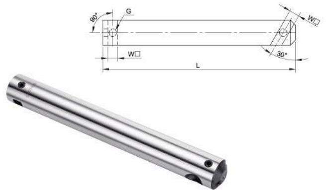
BS 直柄搪孔刀柄 STRAIGHT SHANK BORING HOLDER
