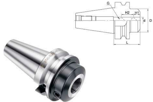
SLA 超短型側固式立銑刀柄 THE SHORTEST SIDE LOCK END MILL HOLDER/SLA
