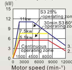
High-speed winding output (Δ connection)
