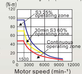
High-speed winding torque (Δ connection)
